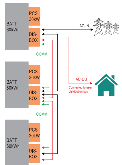
Topology (Max.power ≤ 100 kW)
